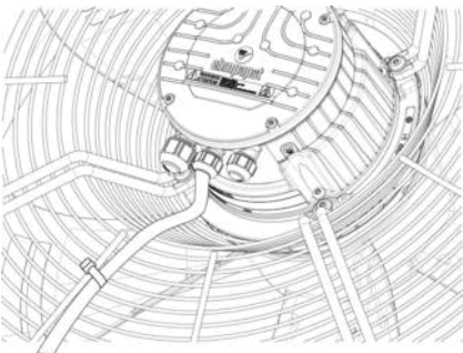
Fig. 1: Fan installed lying flat, cable routed in a U-shaped loop.
